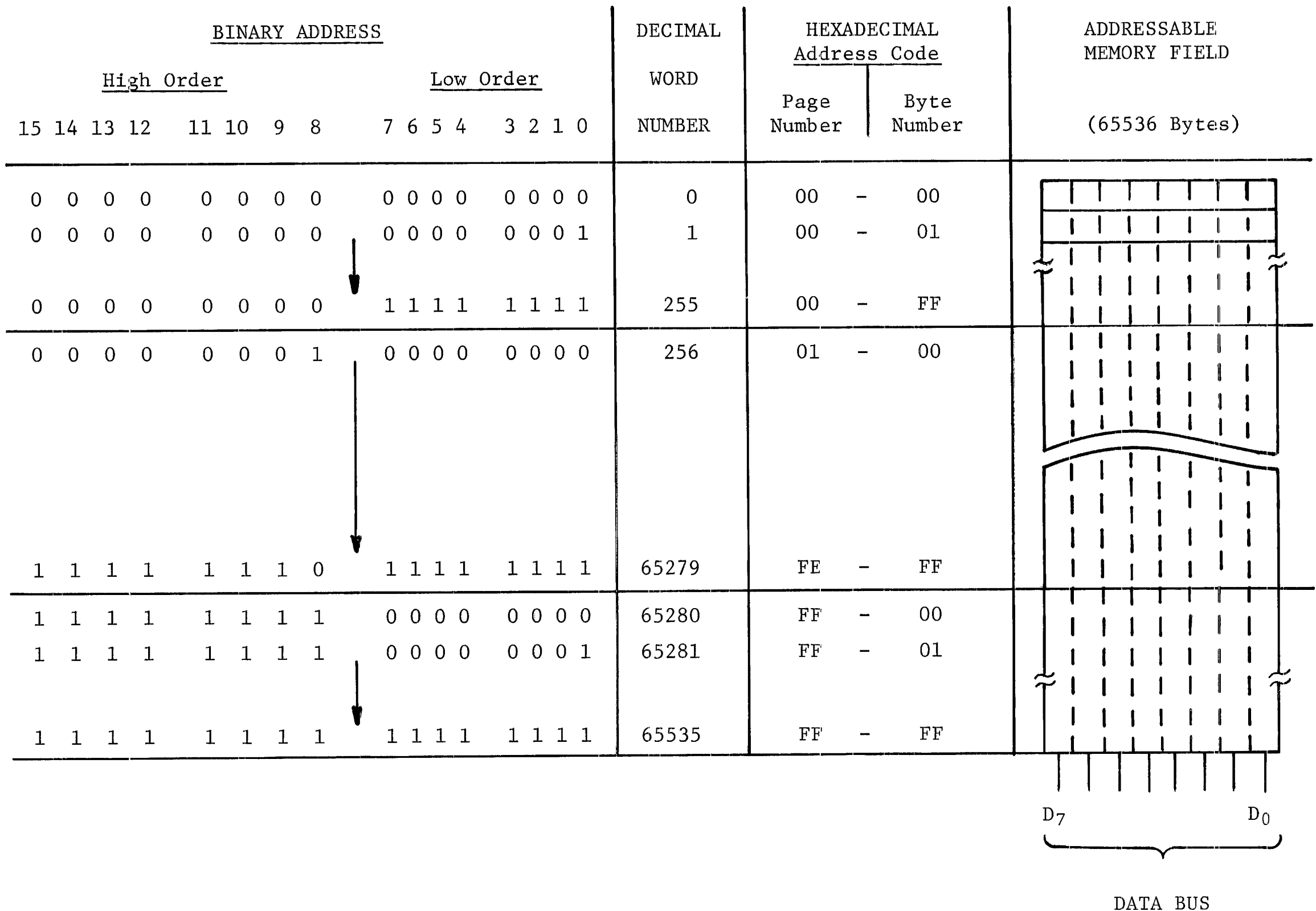
Address Bus and Relation to Memory Field
